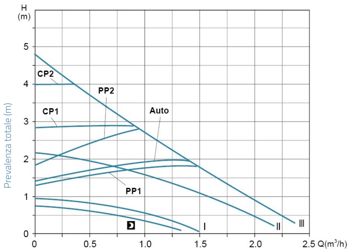
ARPXX-50 Q-H
